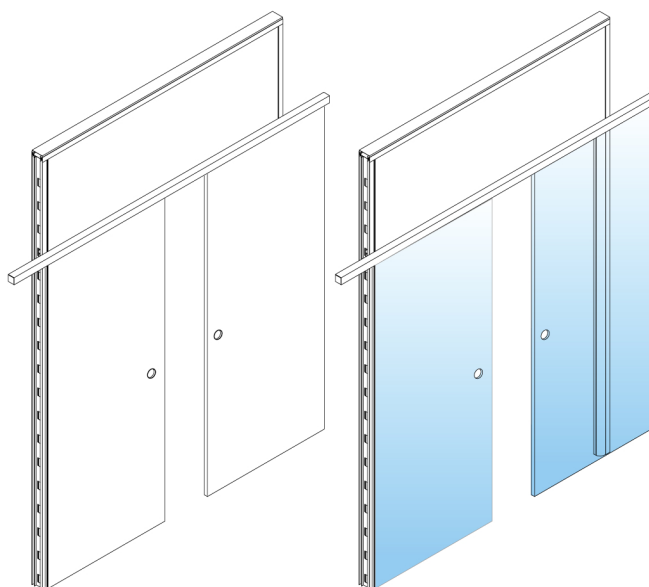
sliding rail for blind door binario scorrevole per porta cieca
