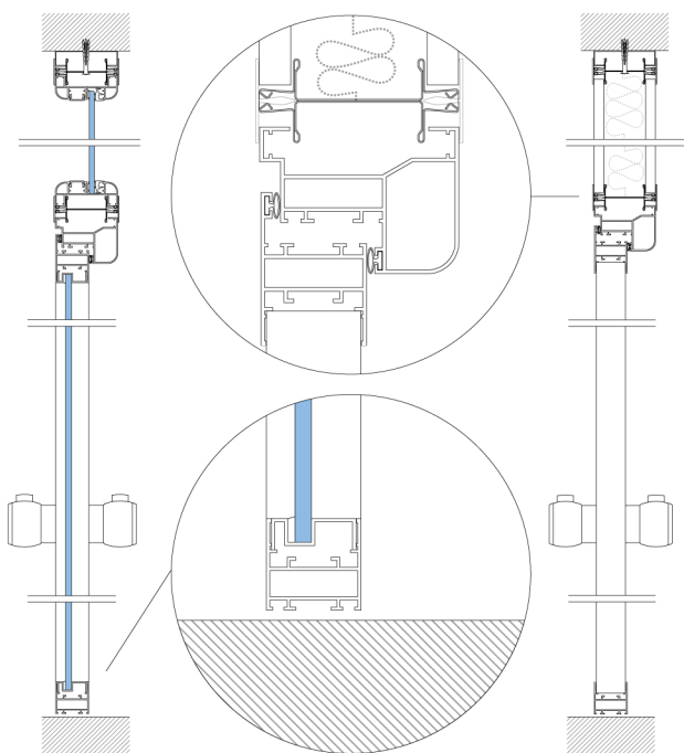
sliding rail for blind door binario scorrevole per porta cieca
